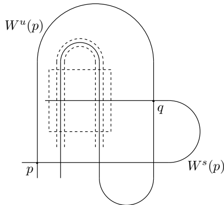
Figure 7: Homoclinic point
