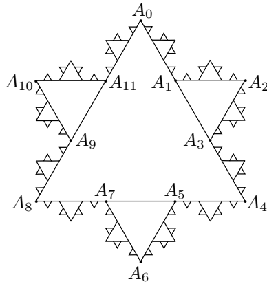
Figure 8.4: Snowflake
