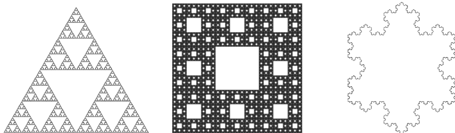
Figure 4: Sierpinski gasket, Sierpinski carpet & the boundary of von Koch snowflake
