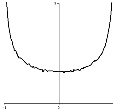
Figure 1.1: The plotted density of an invariant measure for T(x) = 2x^2 - 1 .
