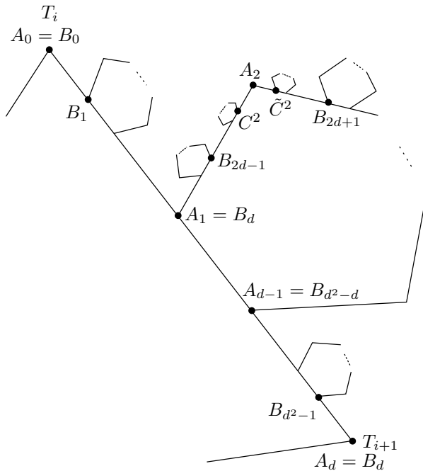
Figure 8.7: Carleson's domain
