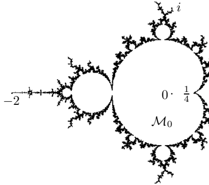
Figure 5.1: Mandelbrot set
